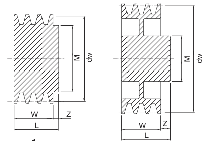
4A (with lightening bores)
