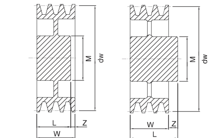
5A (with lightening bores) 8 (3 spokes) 8A (6 spokes)
